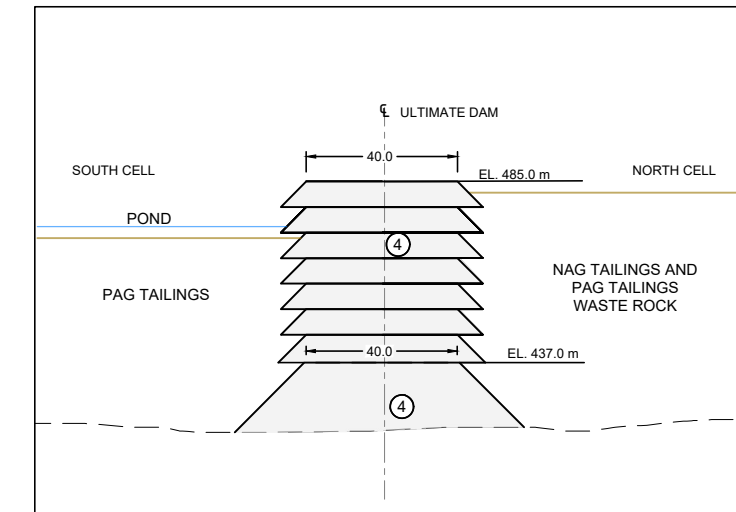
SECTION 3 INTERNAL DAM TYPICAL SECTION SCALE: 1:1000
