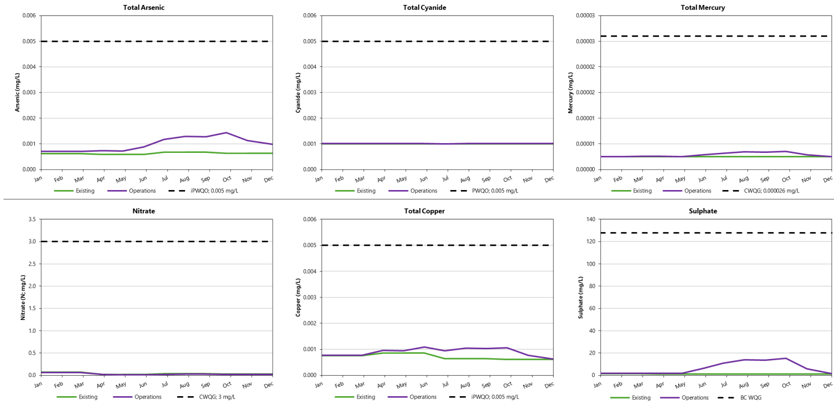
Figure 6.8-6: Springpole Lake, Southeast Arm Water Quality, Eff. Discharge Location (operations)
