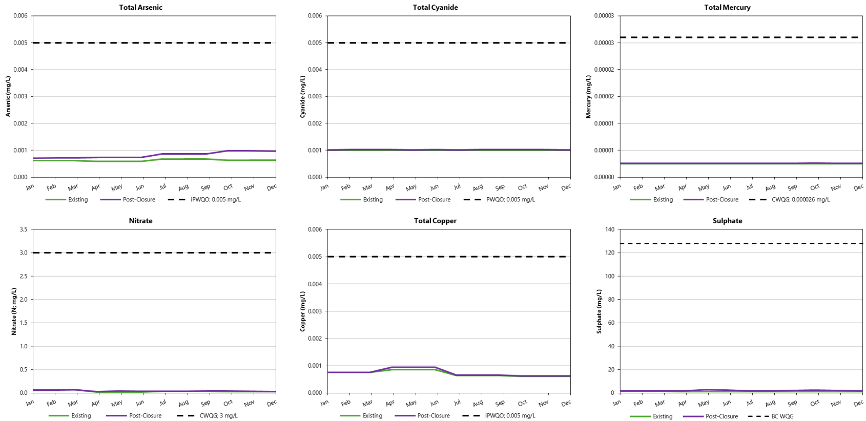
Figure 6.8-9: Springpole Lake, Southeast Arm Water Quality, Node 9 (post-closure)
