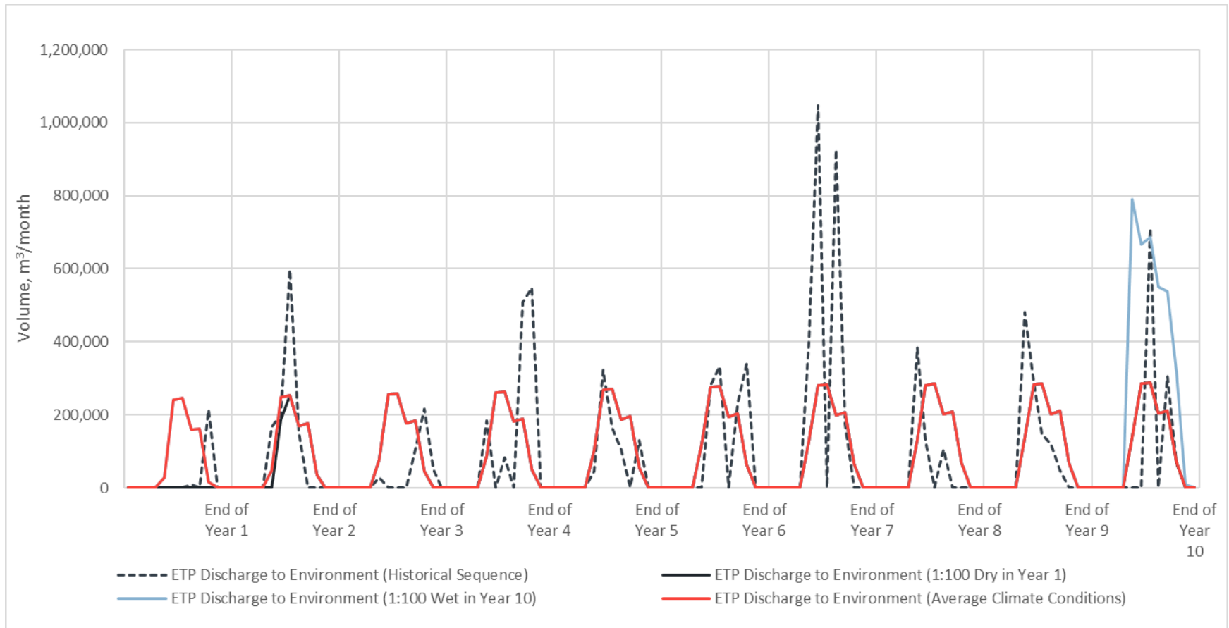
Figure 6.8-4: Treated Effluent Discharge Volume, Operations
