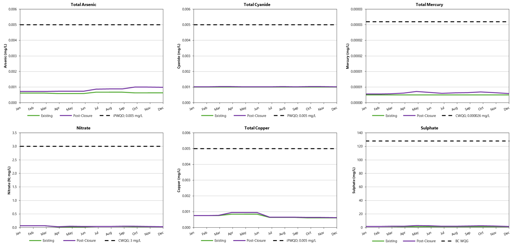
Figure 6.8-7: Springpole Lake, Southeast Arm Water Quality, Eff. Discharge Location (post-closure)
