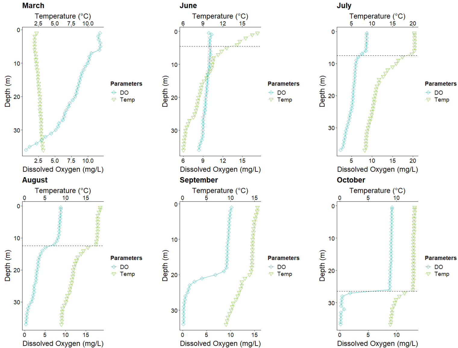
Figure A3-7: Temperature-DO profiles for Birch Lake station BIRCH-B1
