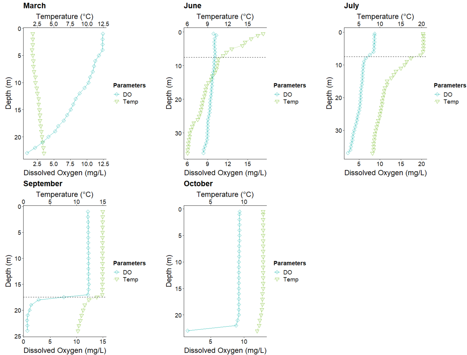
Figure A3-8: Temperature-DO profiles for Birch Lake station BIRCH-B2
