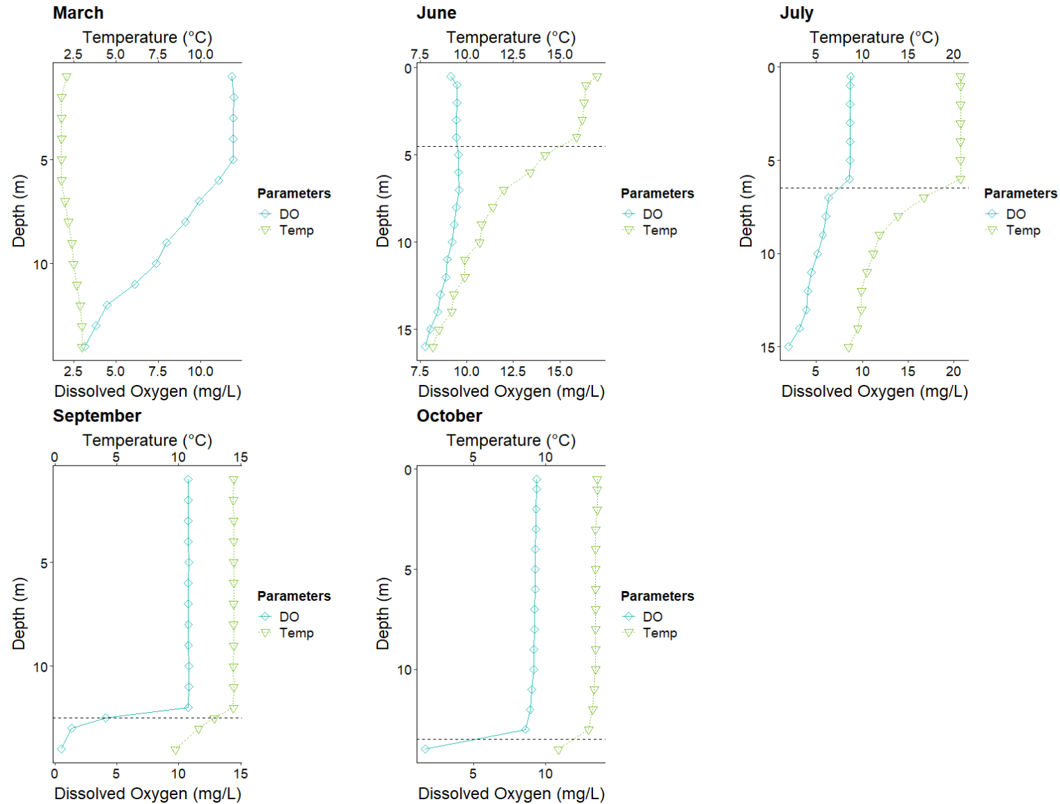
Figure A3-6: Temperature-DO profiles for Springpole Lake station L-15-B6
