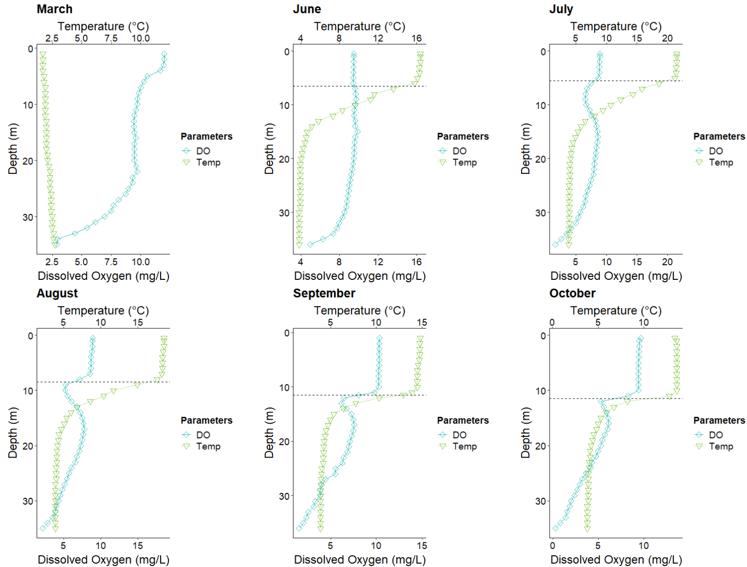
Figure A3-1: Temperature-DO profiles for Springpole Lake station L-15-B1
