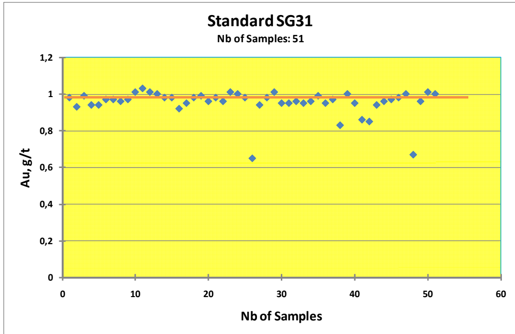
Figure 16.20 Standard SG31
