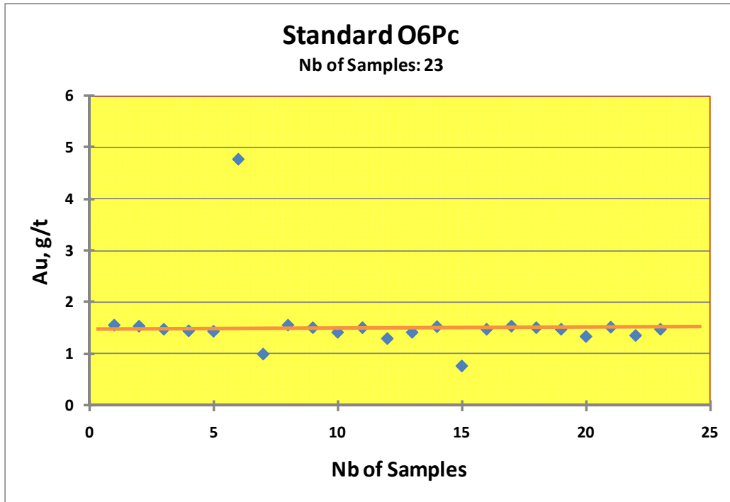
Figure 16.16 Standard O6Pc
