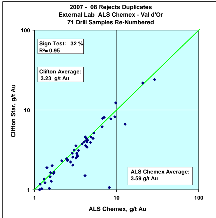
Figure 16.5 2007-08 Rejects Duplicates
