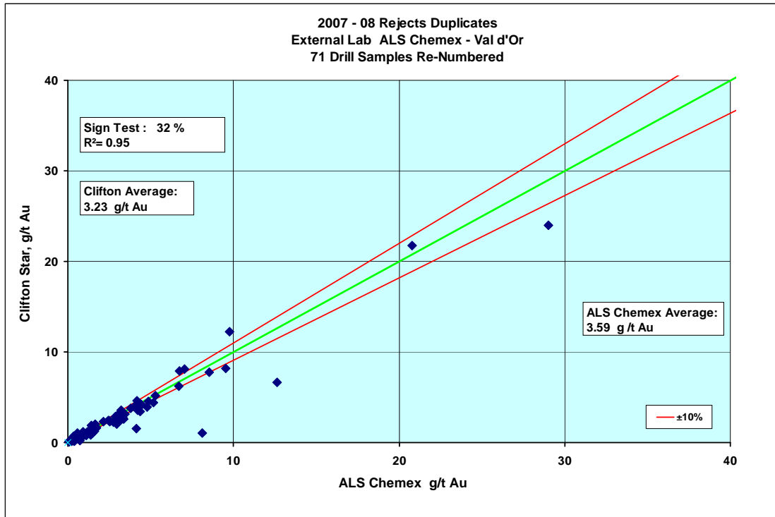
Figure 16.4 2007-08 Rejects Duplicates
