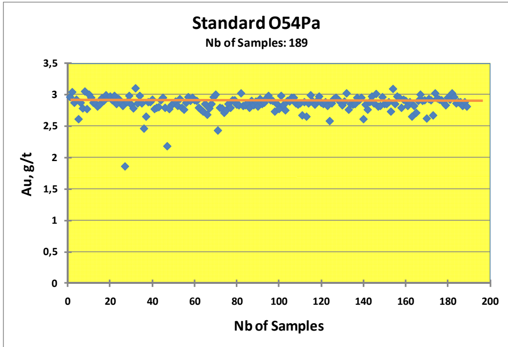
Figure 16.12 Standard O54Pa
