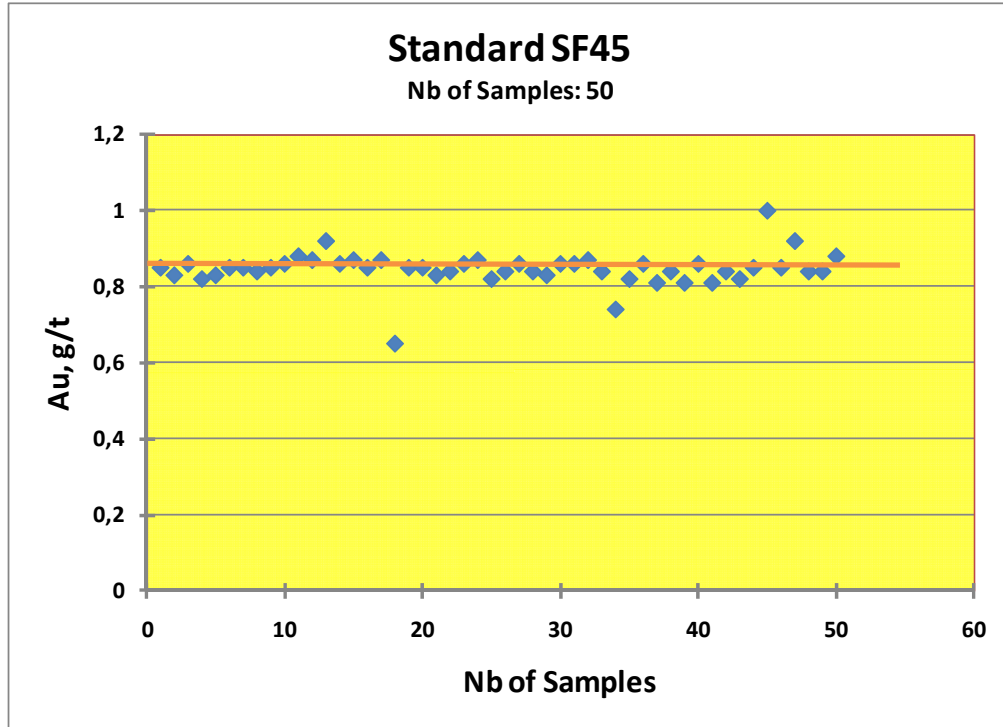
Figure 16.18 Standard SF45
