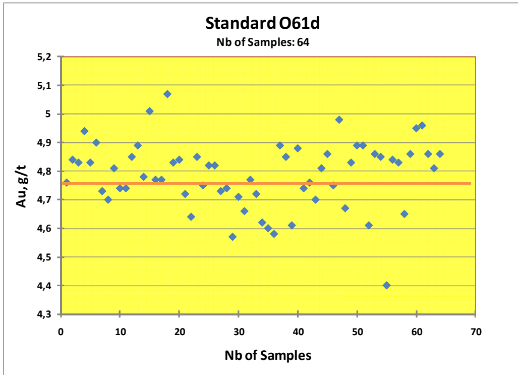
Figure 16.14 Standard O61d
