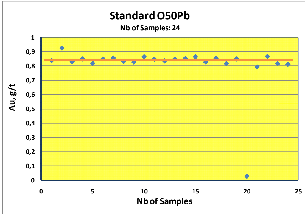
Figure 16.6 Standard O50Pb
