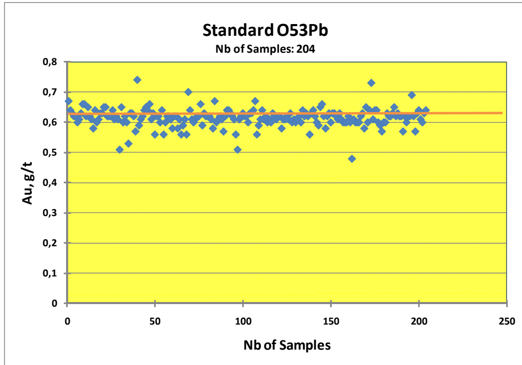
Figure 16.10 Standard O53Pb
