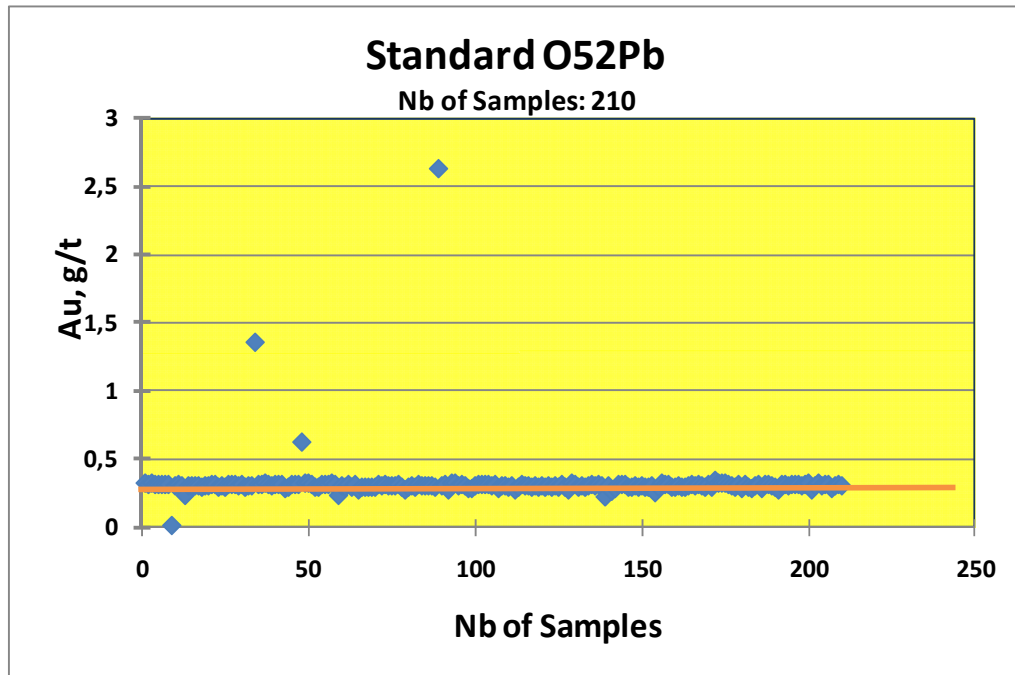
Figure 16.8 Standard O52Pb
