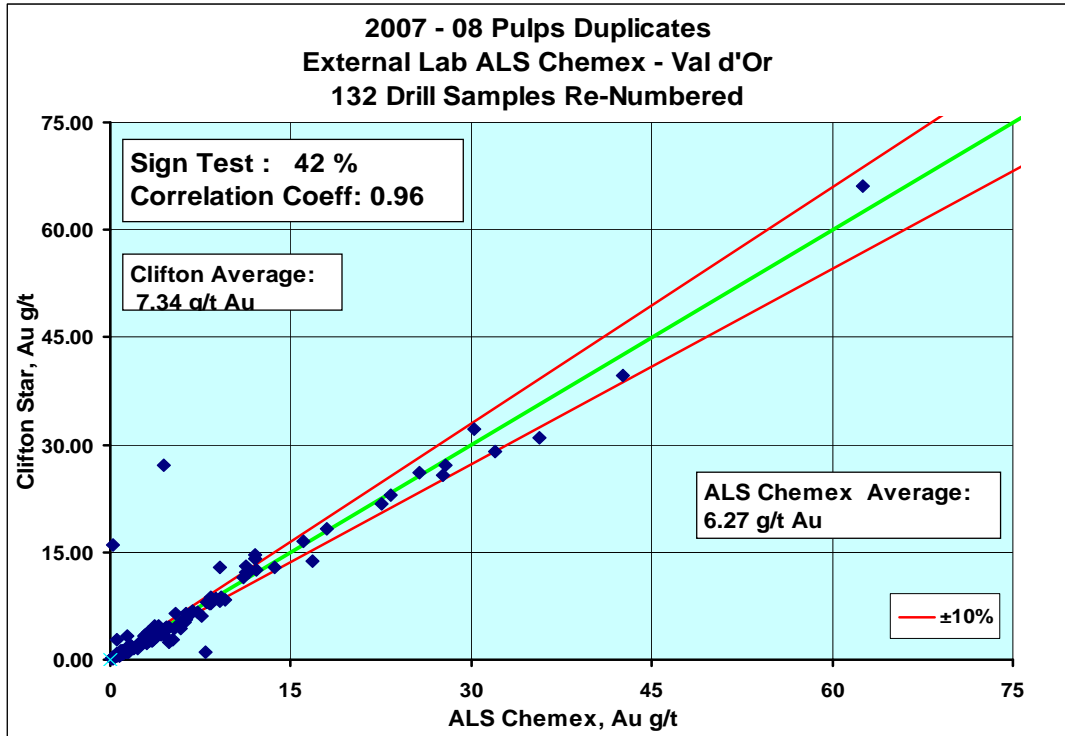
Figure 16.3 2007-08 Pulps Duplicates
