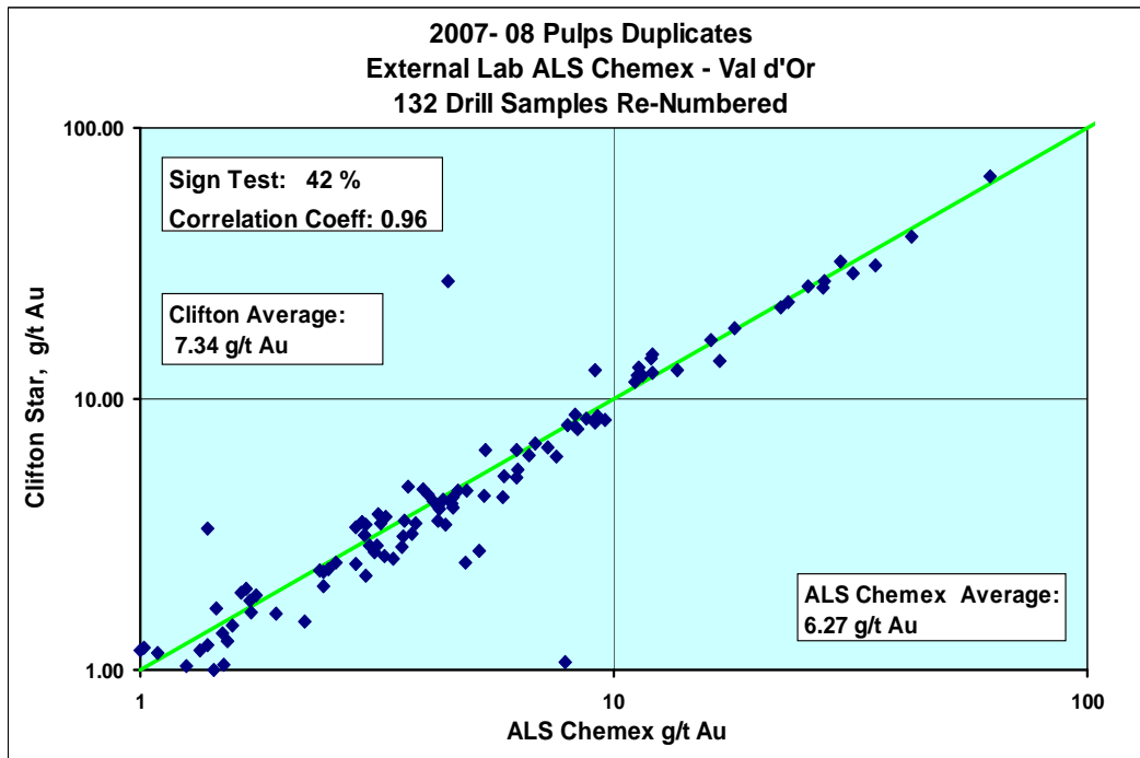
Figure 16.3 2007-08 Pulps Duplicates
